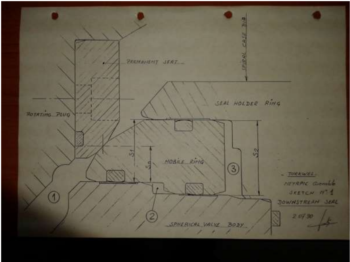
Fig 4: sketch showing part cross section of MIV mobile ring and stationary ring in working position.
