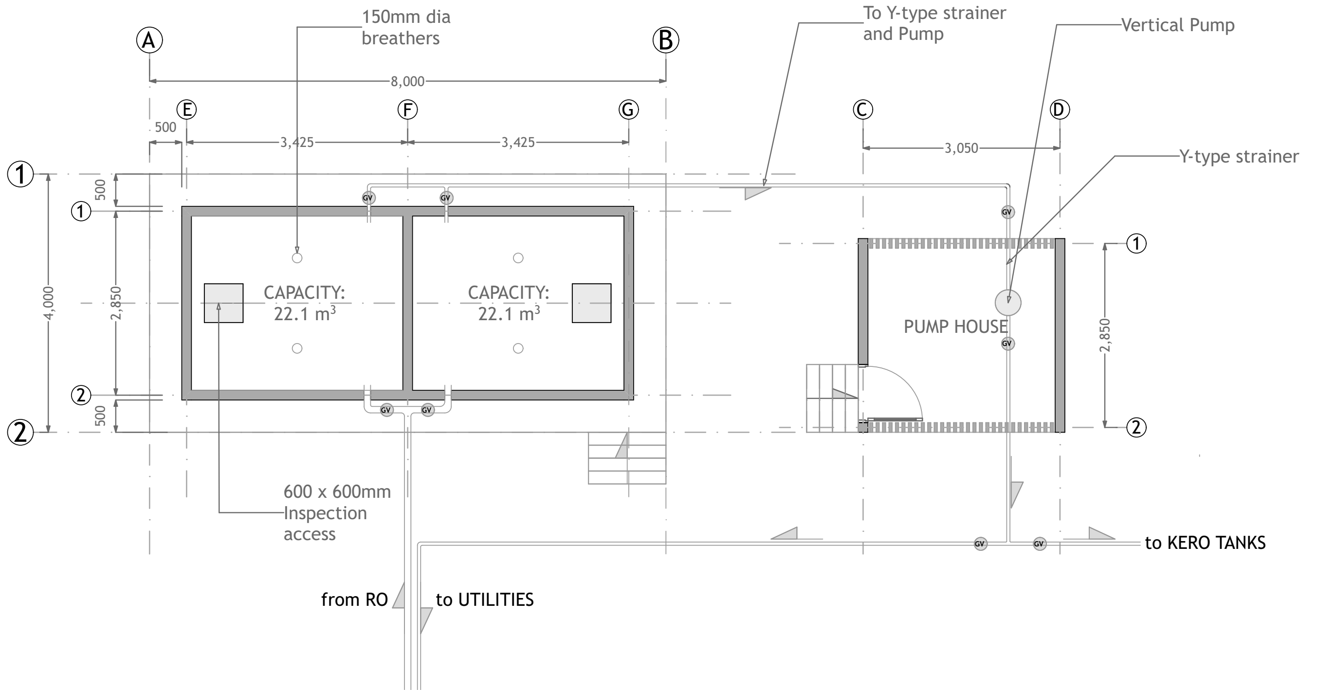
WATER RECOVERY SYSTEM LAYOUT PLAN
