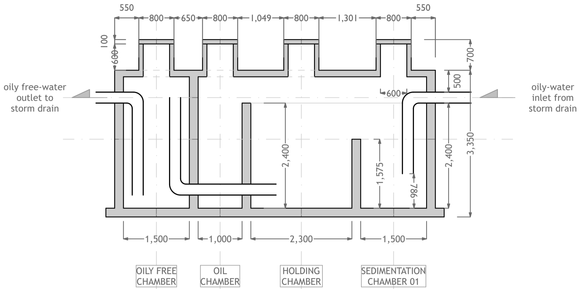
OILY - WATER SEPARATOR INTERCEPTOR SECTION A-A
