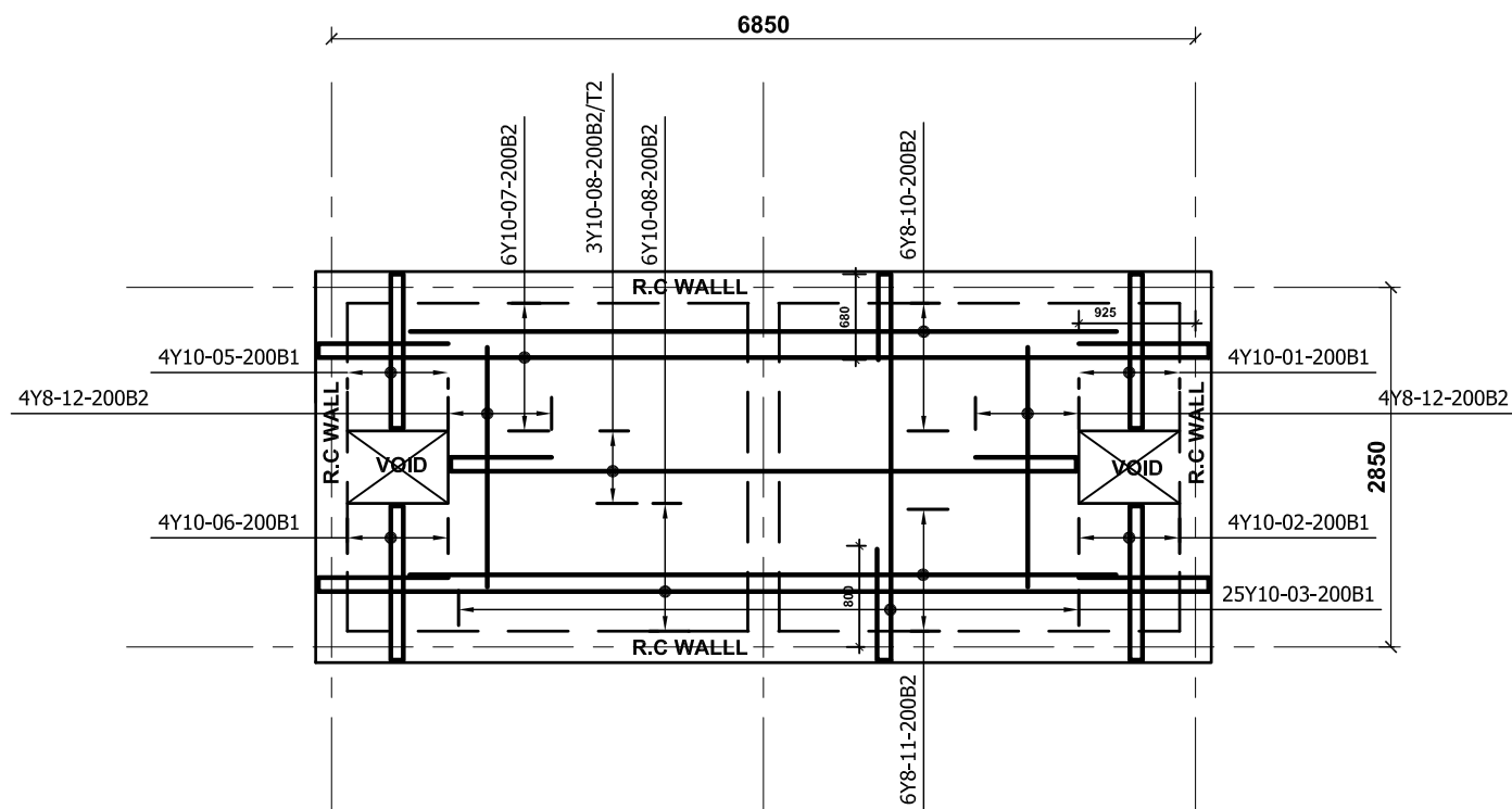
(200mm THICK) SUSPENDED SLAB ,SCALE:1:50
