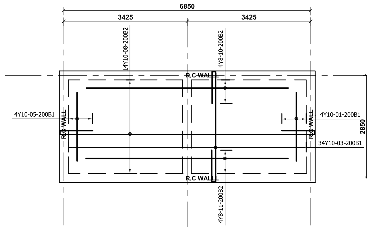
GROUND SLAB PLAN ,SCALE:1:50
