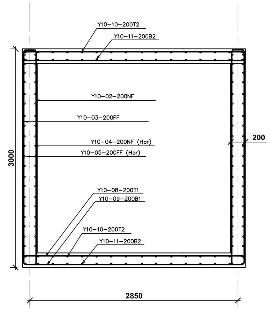
(200mm THICK) SECTION THROUGH THE TANK ,SCALE:1:25
