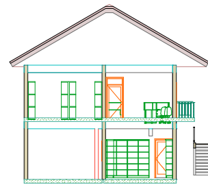
S-03 Building Section 1:100
