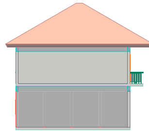
West Elevation 1:100
