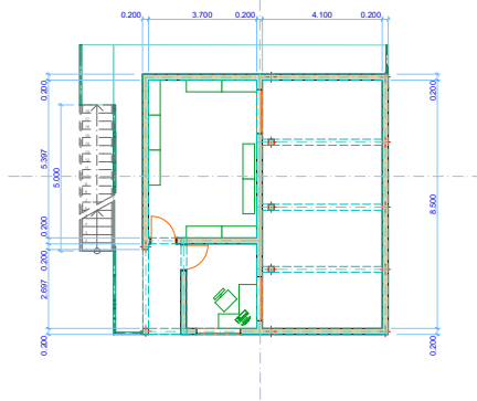
0. Ground Floor 1:100
