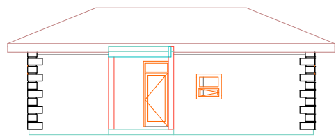
East Elevation 1:100
