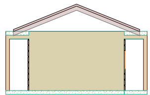
S-01 Building Section 1:100
