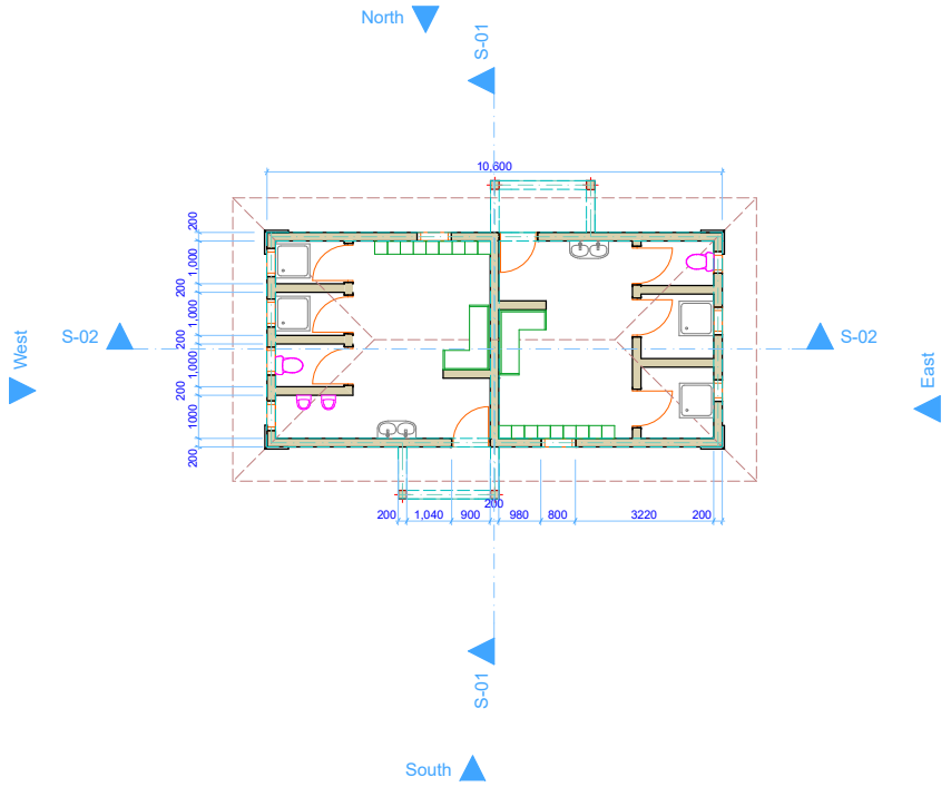
0. Ground Floor 1:100
