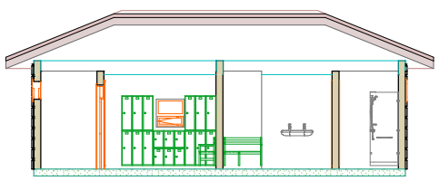
S-02 Building Section 1:100
