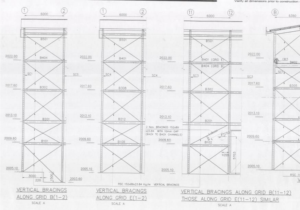
Extract from drawing 2571-101-S-PP-322
